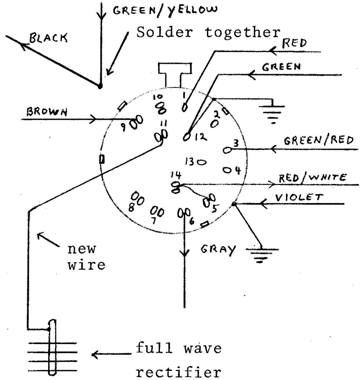
Modified Ignition Switch (Type 2) (Back View)
